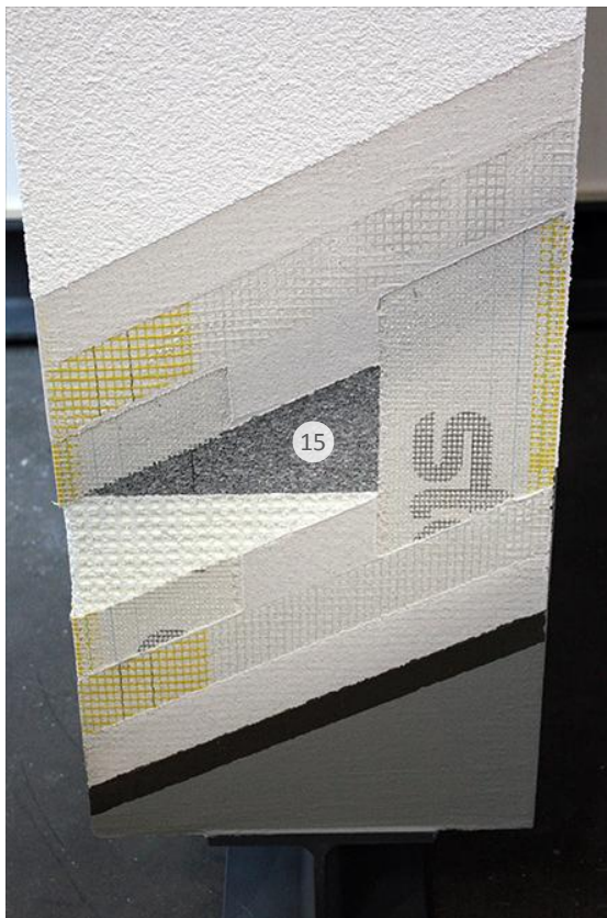
Detail der WDVS-Ebenen Layer detailing of ETICS
